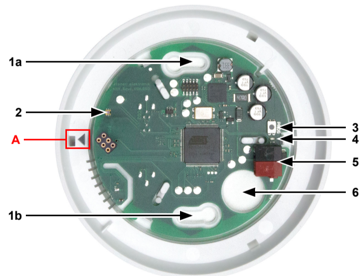
Fig. 2 1 a+b Long holes for mounting (hole distance 60 mm) 2 Brightness sensor 3 Programming button 4 Programming LED 5 KNX-terminal BUS +/- 6 Cable bushing
